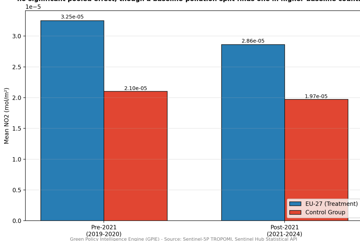
NO 2 : EU-27 vs. 9-Country Control Group, Before vs. After the European Climate Law Two-group DiD model: coefficient = -2.22e-06, p = 0.101 (cluster-robust) - no significant pooled effect, though a baseline-pollution split finds one in higher-baseline countries:
